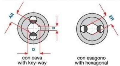
HUB - BORINGS FOR QUICK-RELEASE
